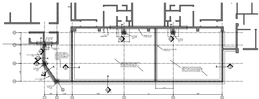
Foundation plan design of proposed addition
